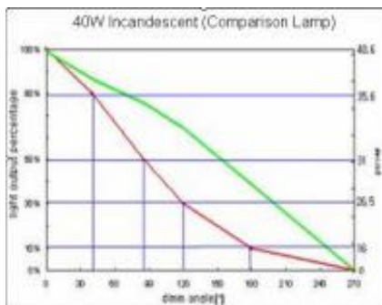
Dimcurve Gloeilamp
